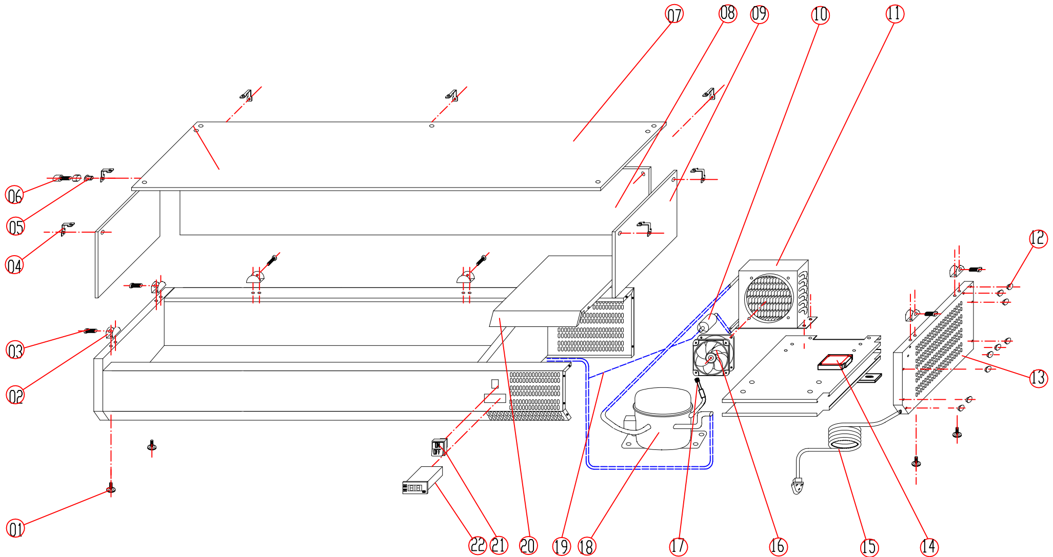
EXPLODED VIEW OF VRX1200,1400,1500,1600,1800,2000/380
